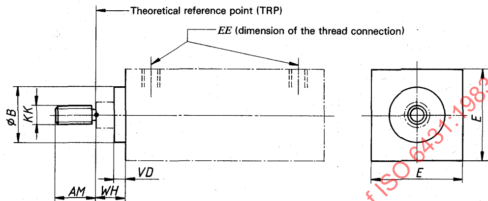
Figure 1 — Basic dimensions
