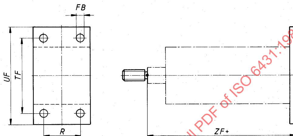
Figure 3 — Cap rectangular flange mounting (MF 2)
