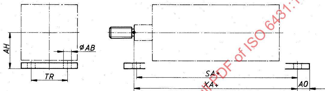
Figure 6 – End angles mounting (MS 1)
