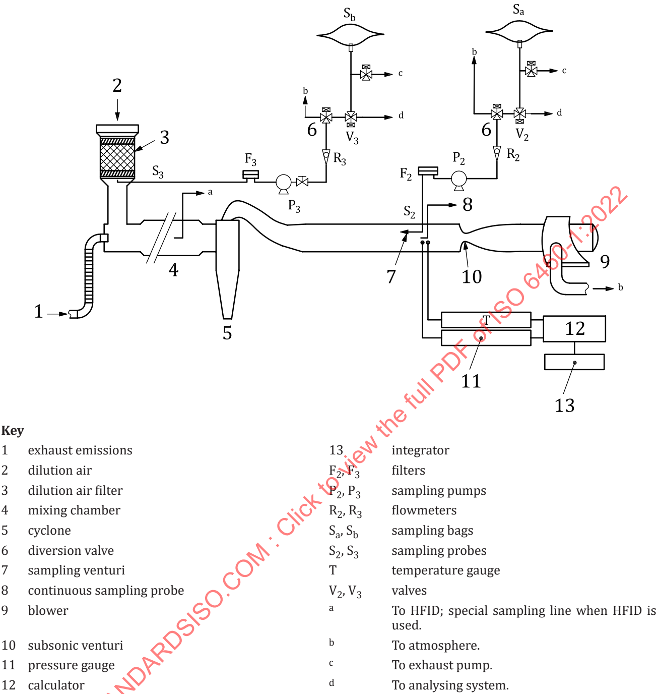
Figure 4— Schematic diagram for the representative closed type CVS system with SSV
