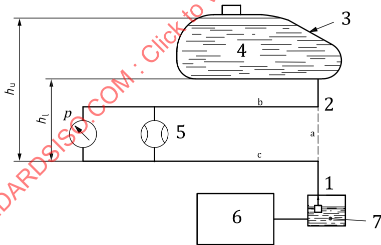
Figure A.2 — Gravimetric method — Carburettor system
