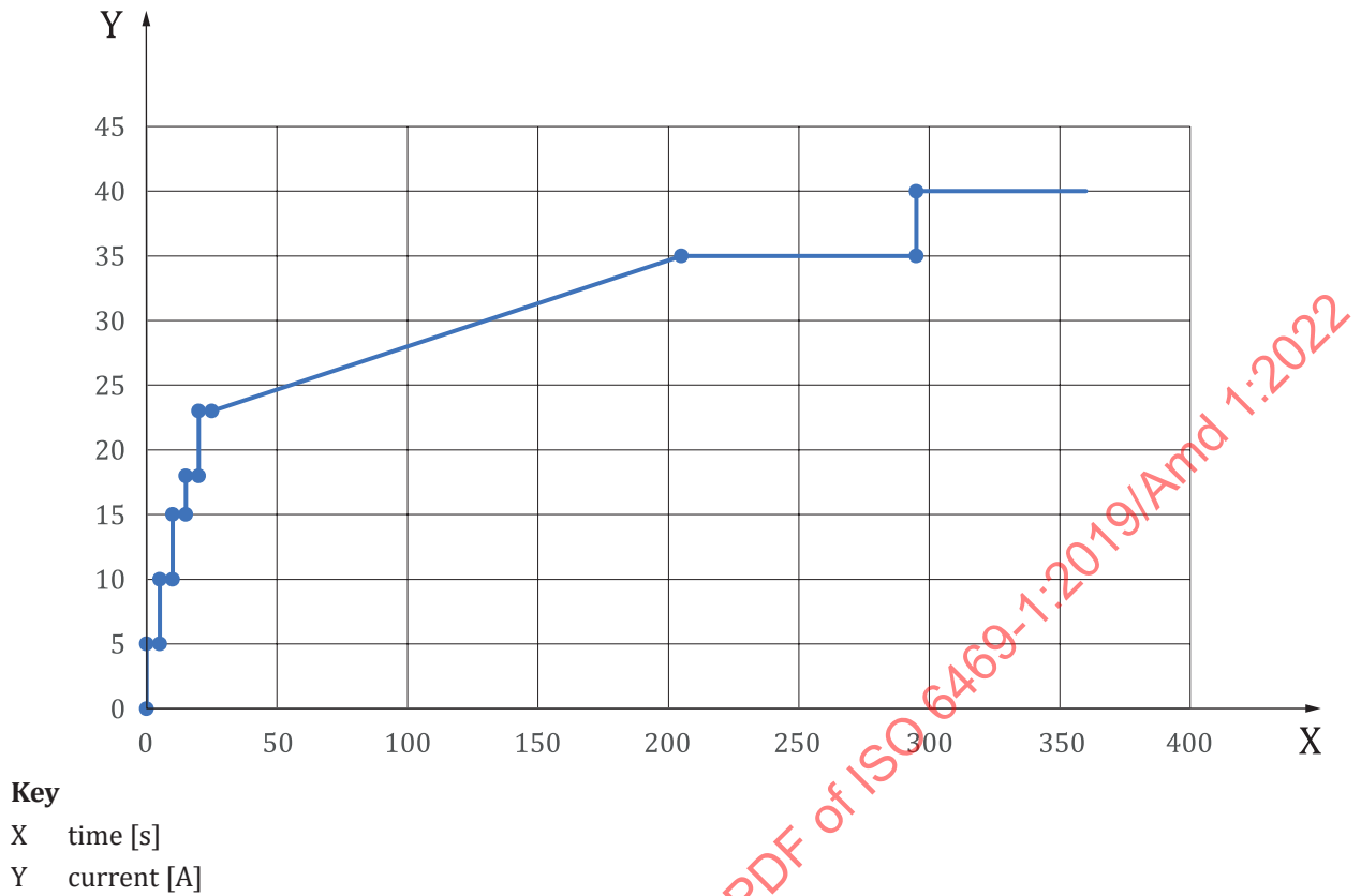
Figure 14 — Current profile for heater
