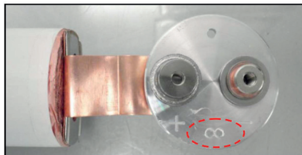
Figure 6 — Example of specific holes in cover for heater connection
