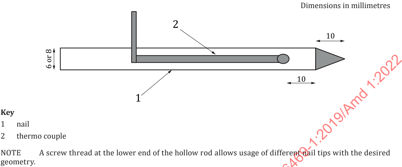
Figure 17 — Example of nail with integrated temperature sensor
