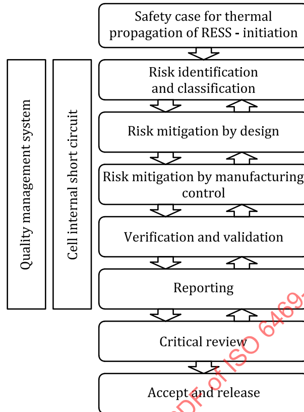
Figure 21 — Developing the safety case for thermal propagation of the RESS
