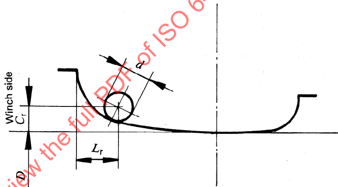
Figure 2 — Dimensions for calculation of shaft torque
