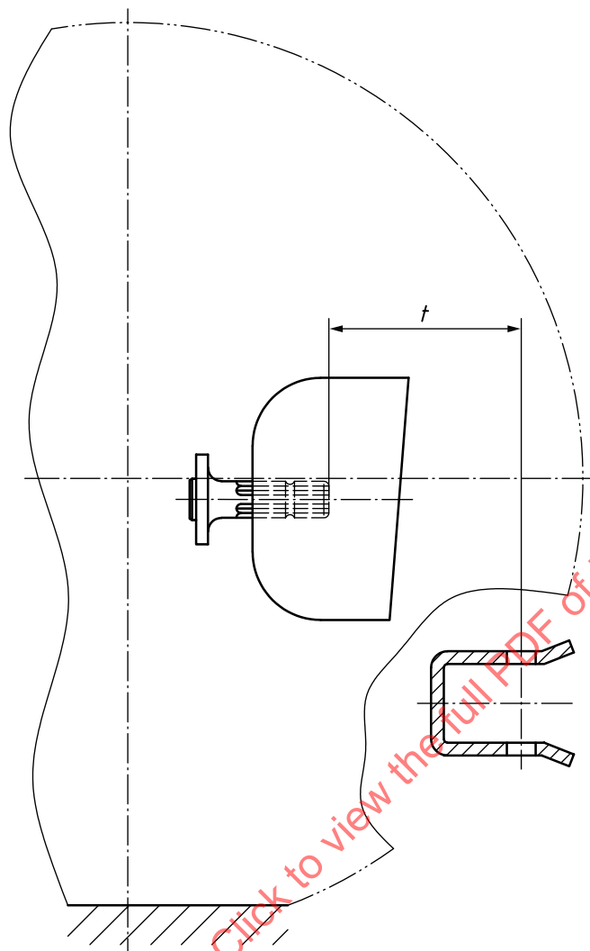
Figure 2 — Non-swivel clevis coupling — Relation to power take-off (PTO)
