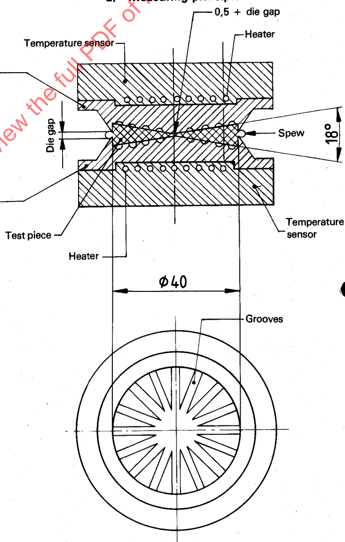
a) Measuring principle
