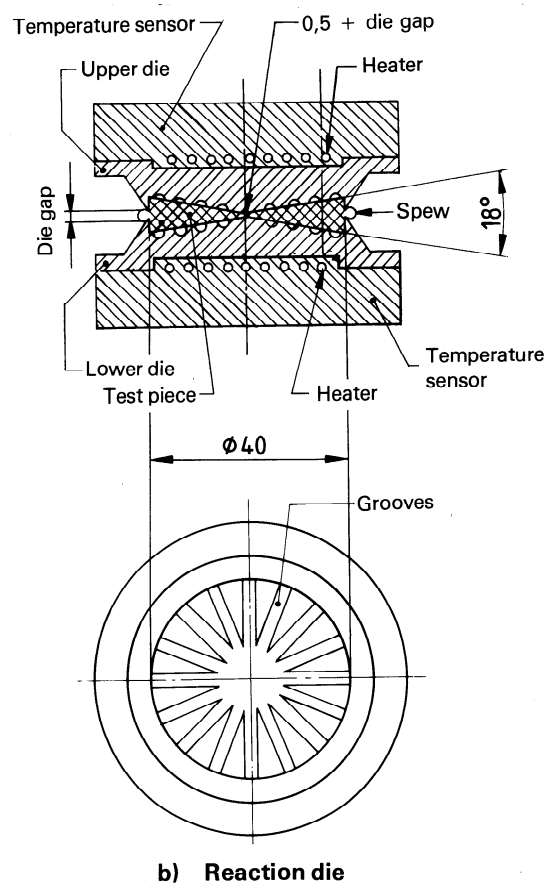
Figure 3 — Typical torsion shear curemeter
