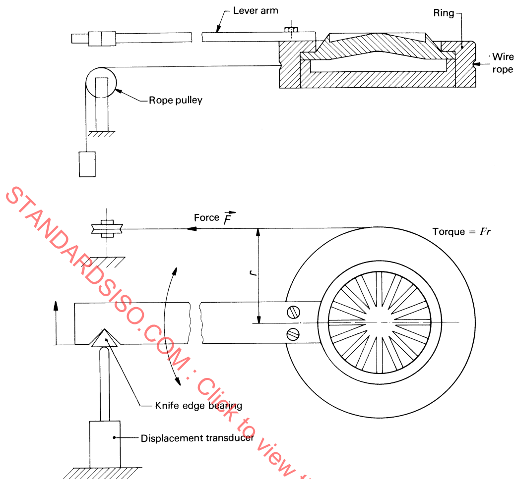
Figure 5 — Calibration equipment for torsion shear curemeter
