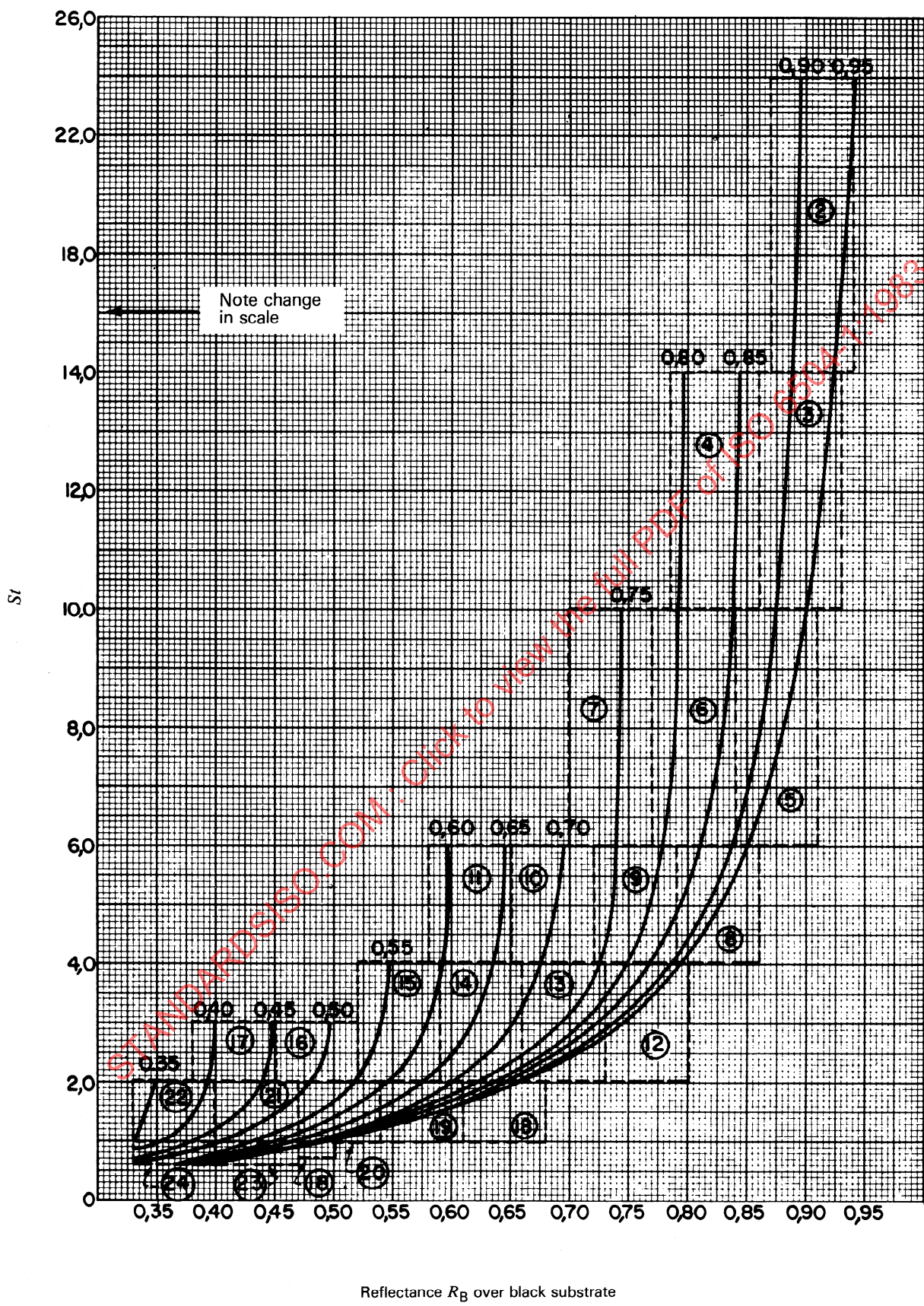
Figure 1 — Index graph for determination of S_l from values of R_B and R_\infty
