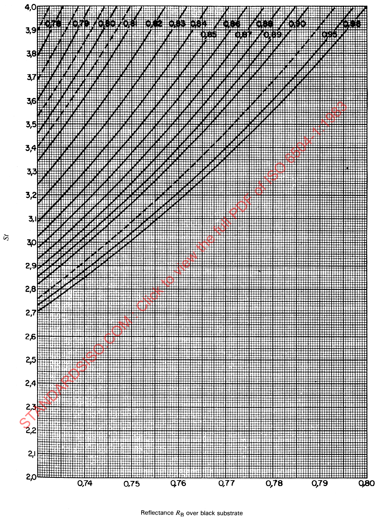
Figure 12 — Values of S_t for the ranges 0,73 \leq R_B \leq 0,80 0,78 \leq R_\infty \leq 0,98
