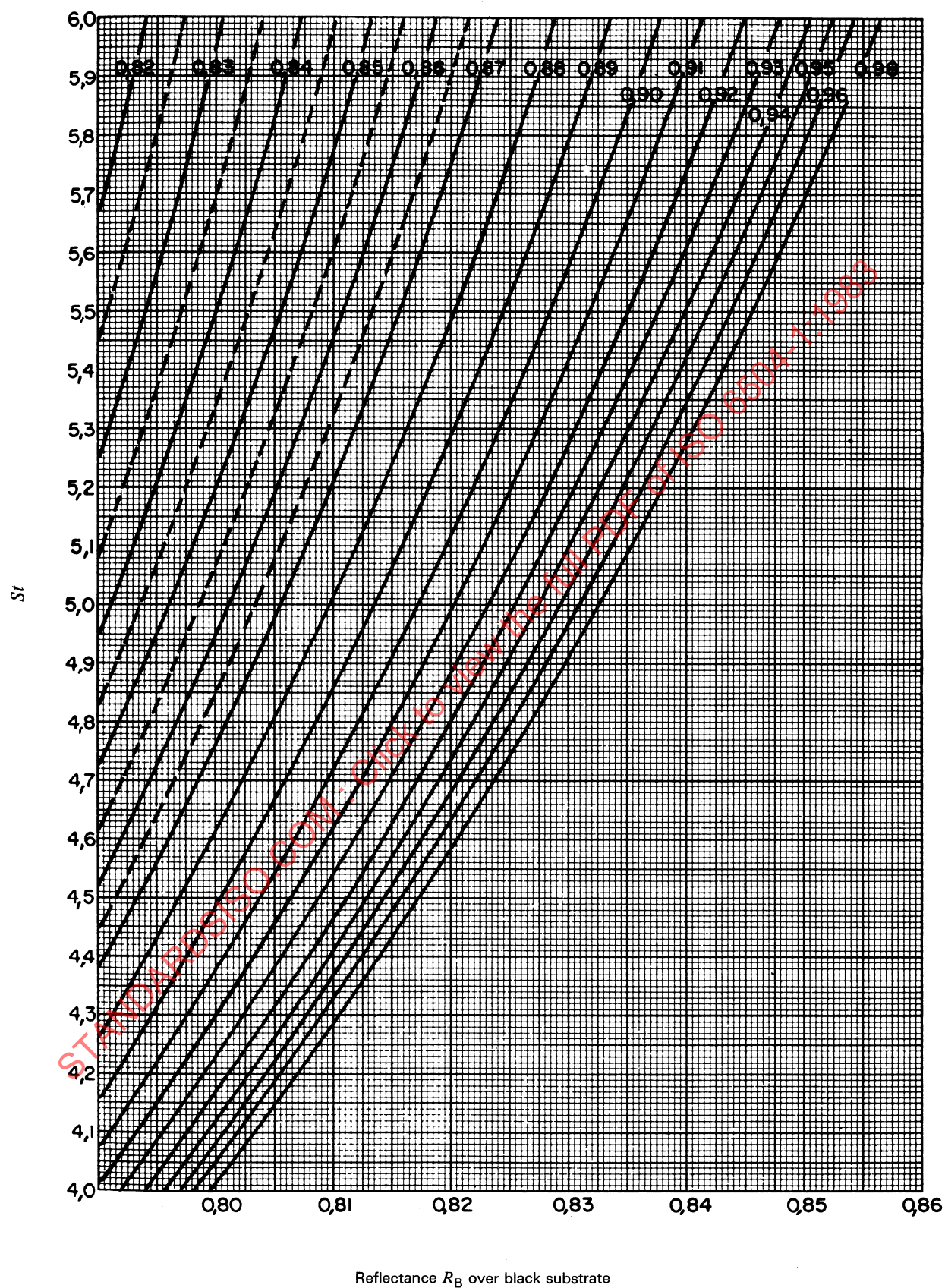
Figure 8 — Values of S_t for the ranges 0,79 \leq R_B \leq 0,86 0,82 \leq R_\infty \leq 0,98
