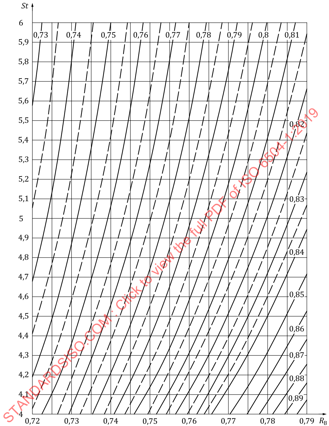
Figure A.9 — Values of St for the ranges 0,72 \leq R_B \leq 0,79 0,73 \leq R_\infty \leq 0,89
