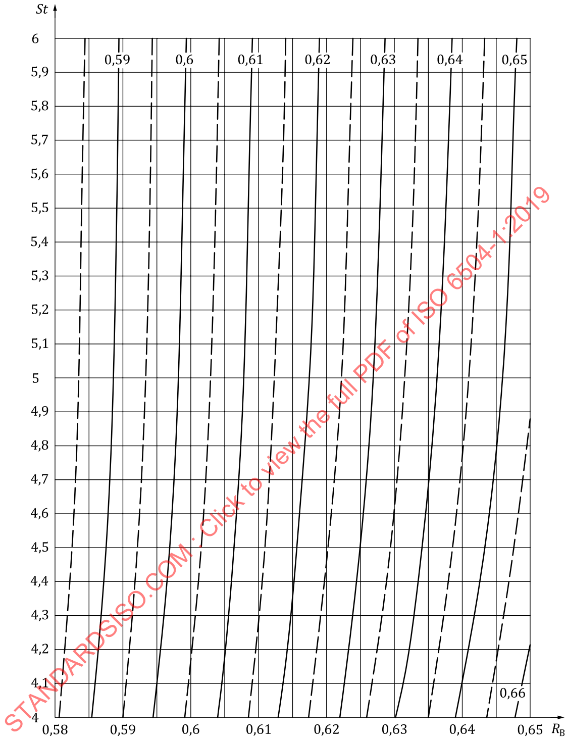
Figure A.11 — Values of St for the ranges 0,58 \leq R_B \leq 0,65 0,59 \leq R_\infty \leq 0,66
