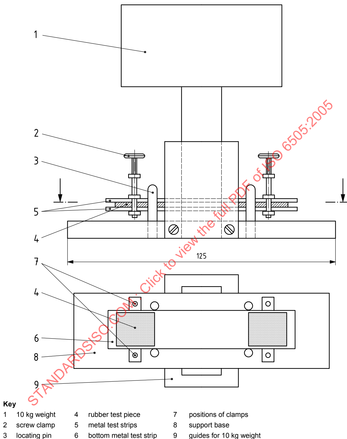
Figure 1 — Typical support jig
