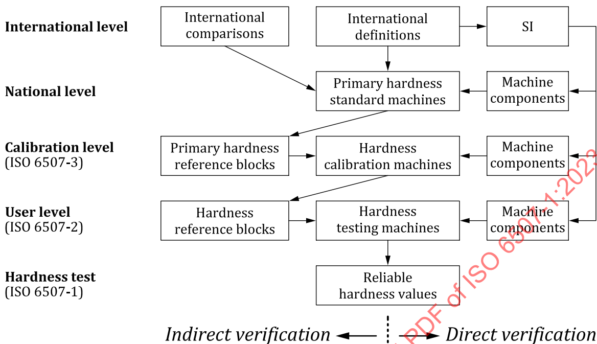
Figure E.1 — Chains of calibrations
