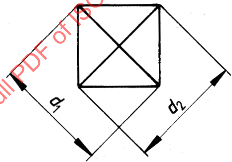
Figure 2 — Vickers indentation
