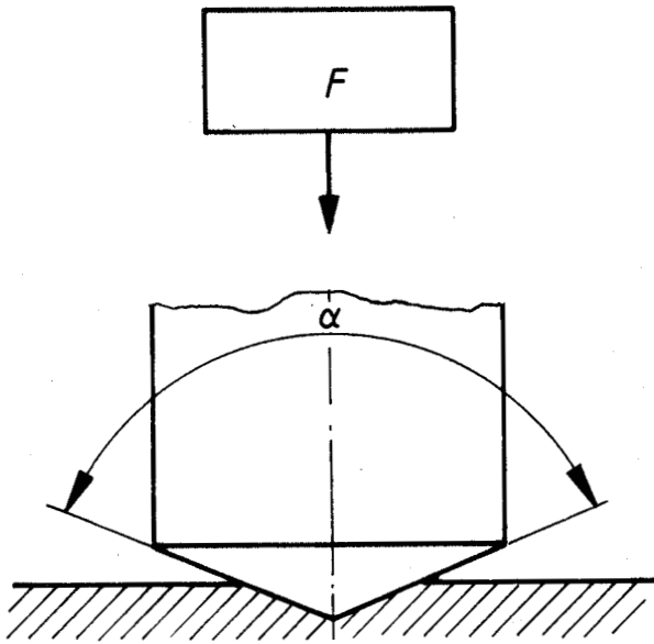
Figure 1 — Indenter (pyramidal diamond)
