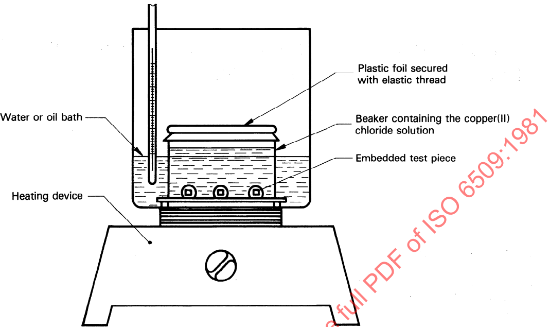
Figure 1 — Example of test apparatus
