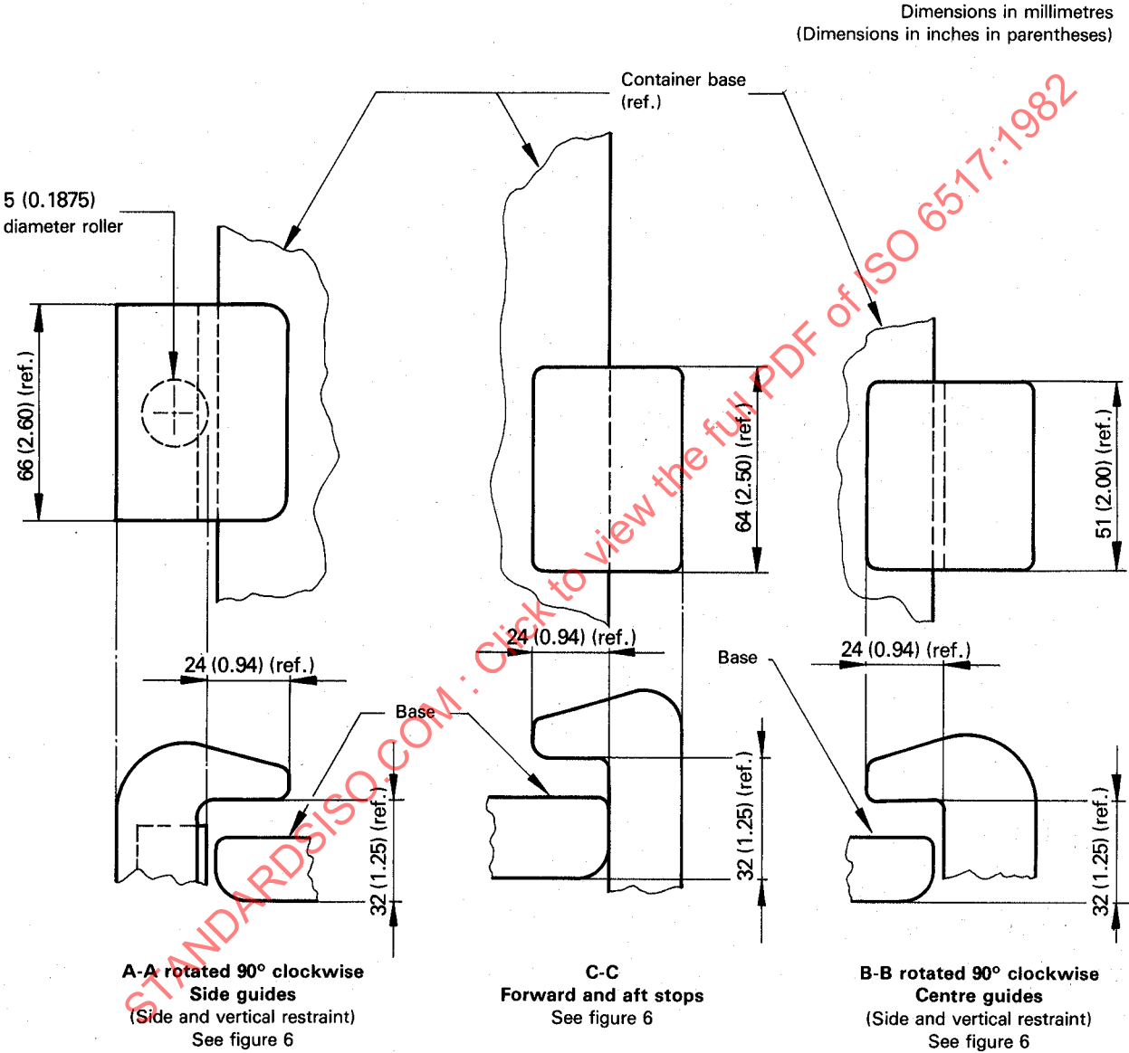
Figure 5 — Restraint details
