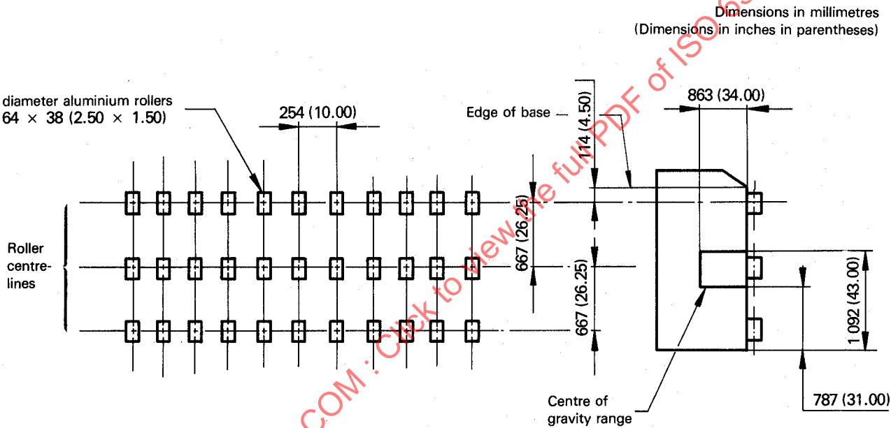
Figure 7 — Static test roller patterns
