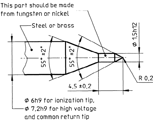
Figure 6 — Spark gap electrode requirements
