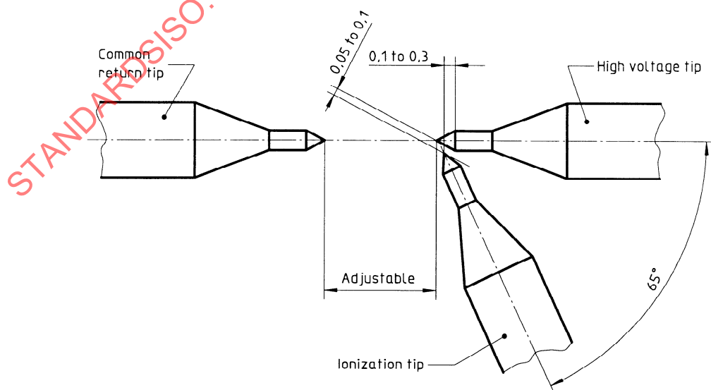
Figure 5 — Setting of pointed spark gap
