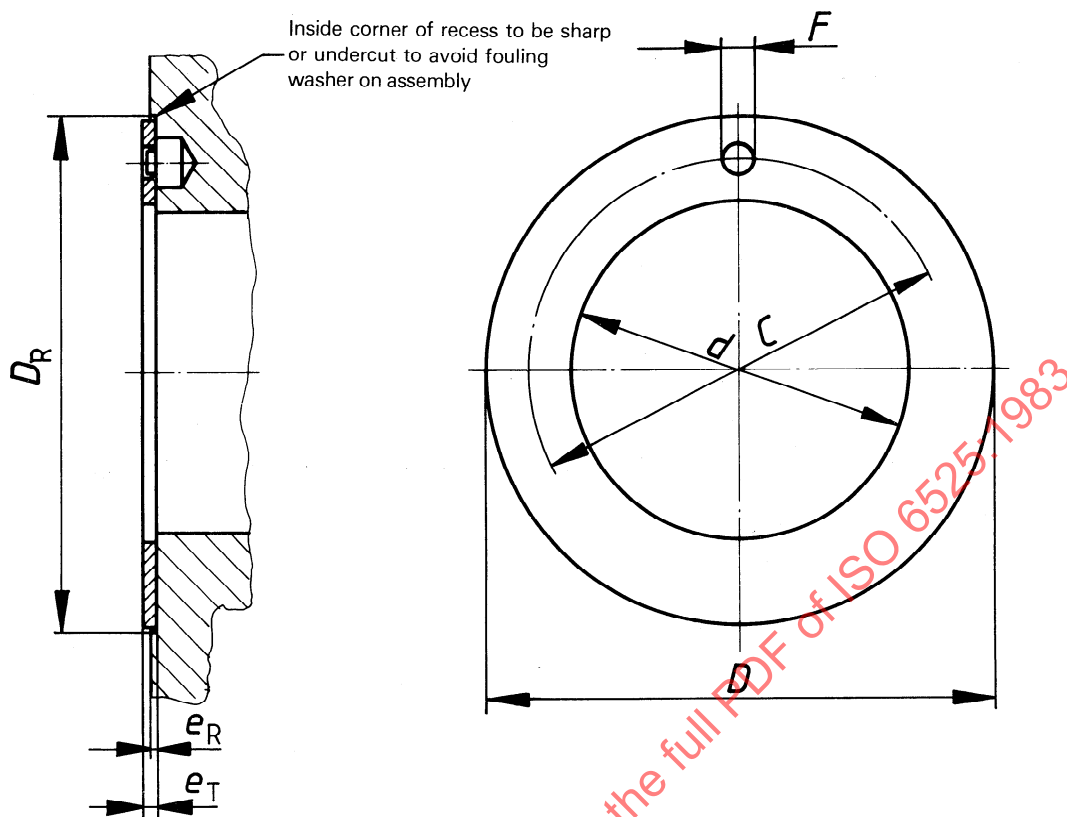
Figure 1 — Thrust washer
