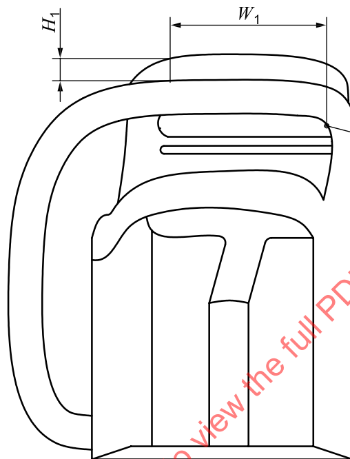
Figure 4 — Front hand-guard width, W_1 , from the rear view of the machine
