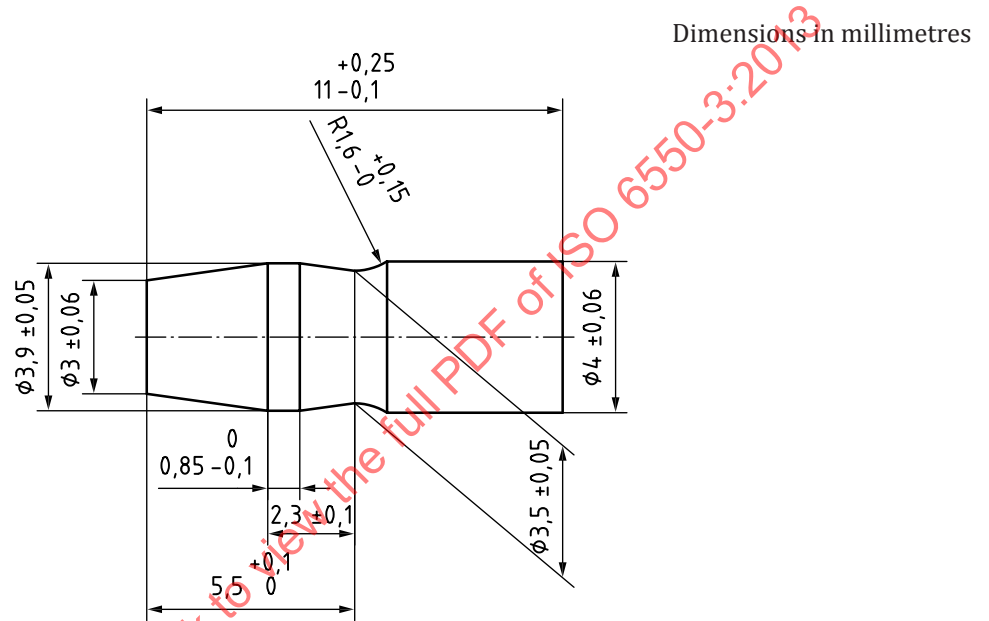
Figure A.1 — Pin terminal dimensions
