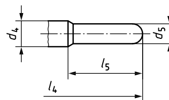
e) With reduced tip end diameter at sheathed glow element b
