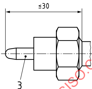
d) With pin terminal b (type C4)
