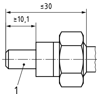
b) With blade terminal b (types B1 and B2)
