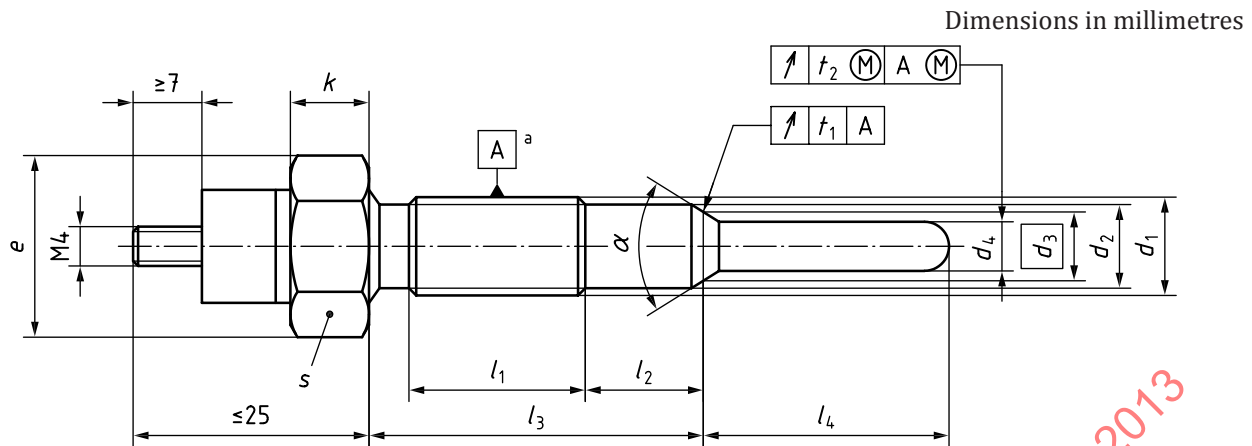
a) With threaded terminal (types A1 to A6 and C1 to C3)
