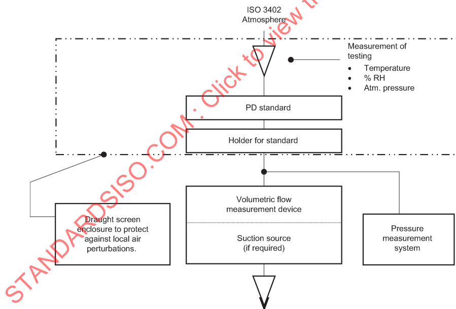
Figure A.2 — Typical arrangement of calibration apparatus
