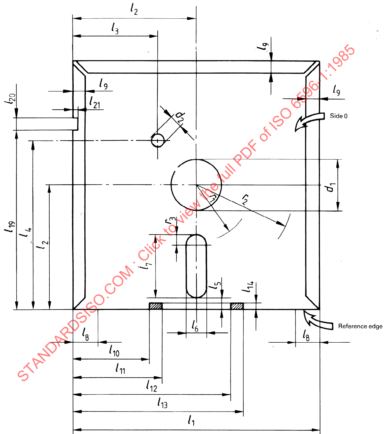
Figure 4 — Jacket dimensions
