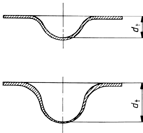
Figure 4 — Examples for the failure criterion "indentation" for two materials of differing toughness
