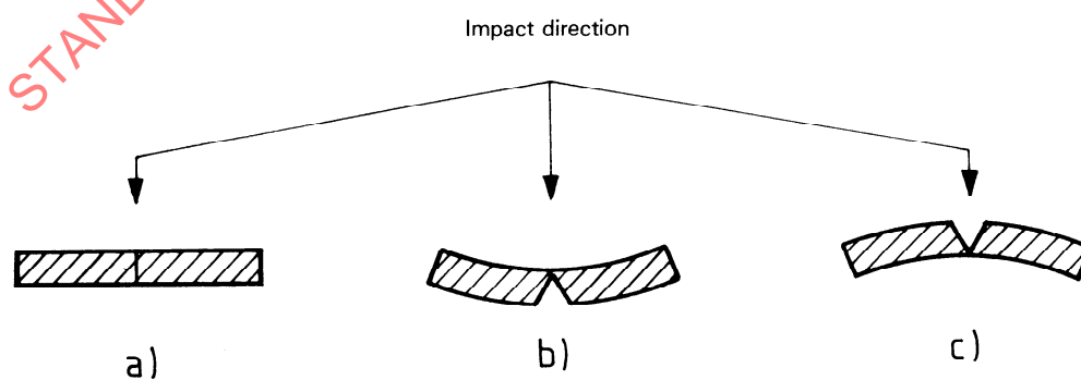
Figure 2 — Sections through specimens damaged by a "break" [b) and c) after bending by hand]
