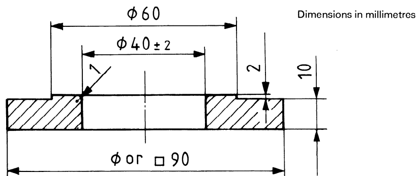
Figure 6 — Test specimen support
