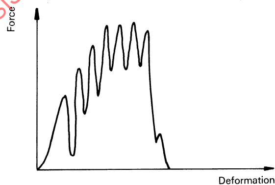
Figure A.3 — Force-deformation diagram in the case of strong resonance (schematic)
