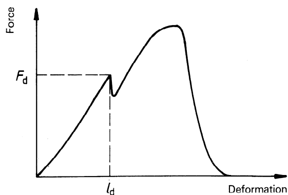
Figure A.1 — Force-deformation diagram for a UV-aged or strongly oriented material (schematic)
