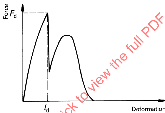
Figure A.2 — Force-deformation diagram for a brittle or fibre-filled material (schematic)
