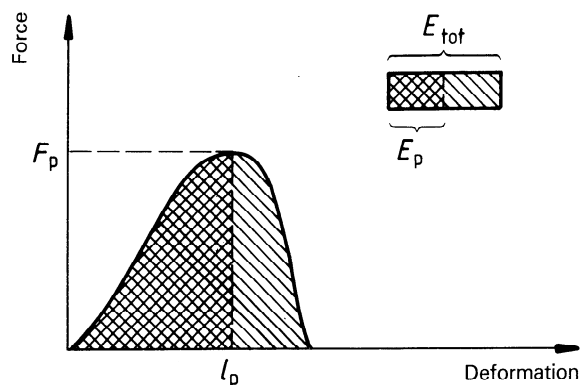
Figure 1 — Force-deformation diagram for tough materials (schematic)
