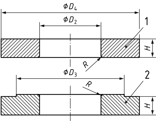
Figure 5 — Example of test device
