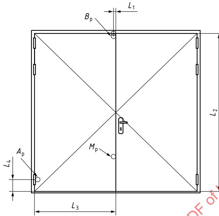
b) Double leaf doors
