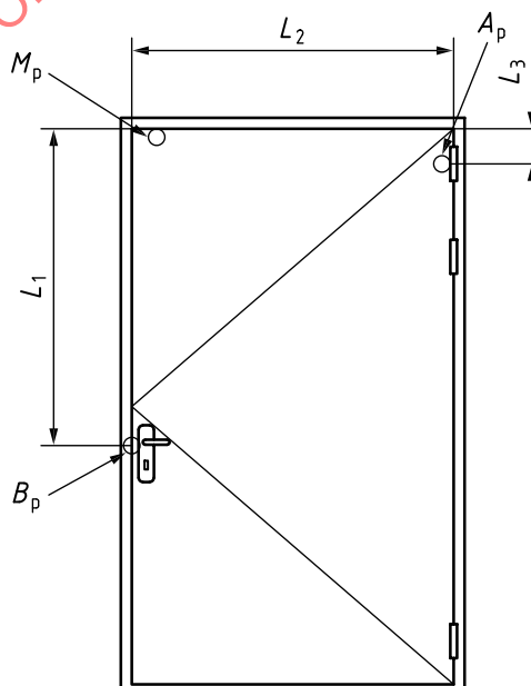
Figure A.3 — Three gauge measurements relative to the frame
