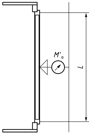
a) Test pressure equal to 0 Pa
