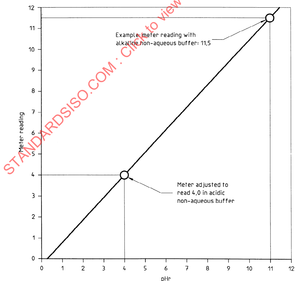
Figure B.1 — Example of calibration curve for conversion of pH meter readings to pHr
