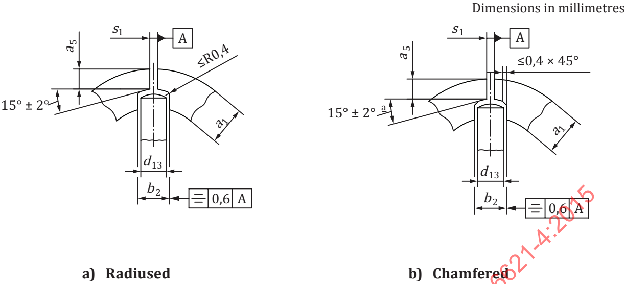
Figure 1 — Internal notch
