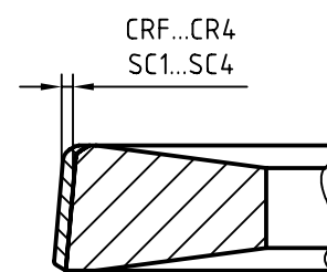
d) TM or KM rings
