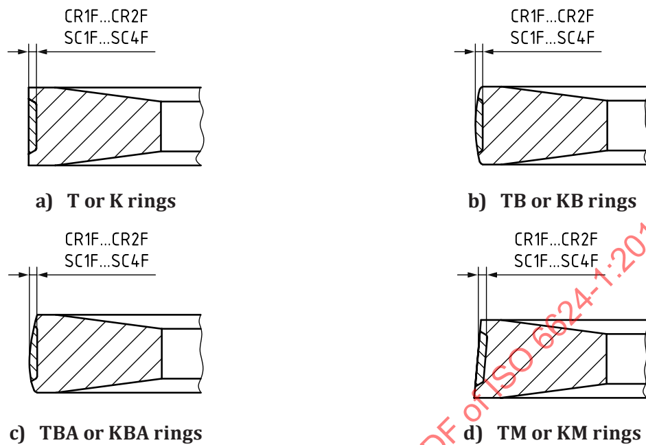
Figure 16 — Inlaid rings
