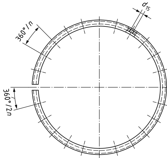
Figure 10 — Arrangement of holes
