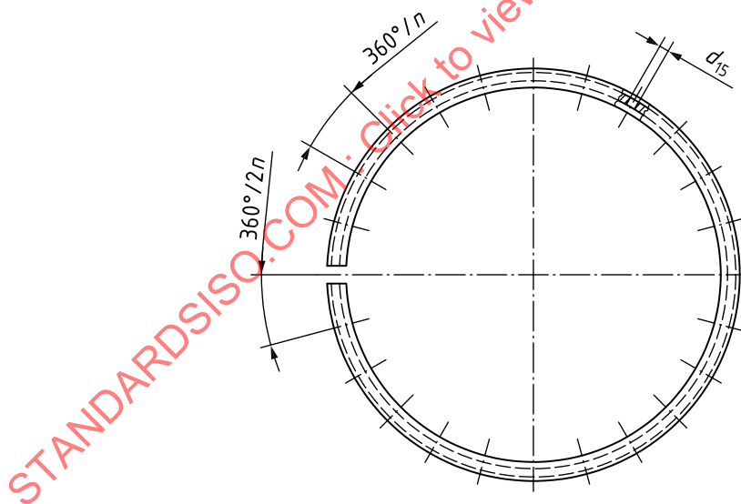
Figure 10 — Arrangement of holes
