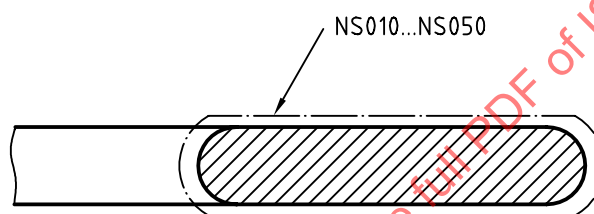
Figure 5 — Nitrided segment
