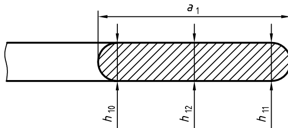
Figure 6 — Segment width
