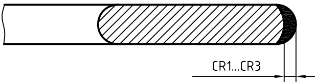
Figure 4 — Chromium-plated segment
