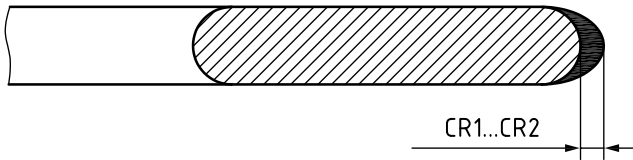
Figure 4 — Chromium-plated rail
