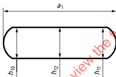
Figure 7 — Rail width
