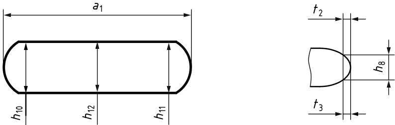
Figure 9 — Rail with barrel face dimension
