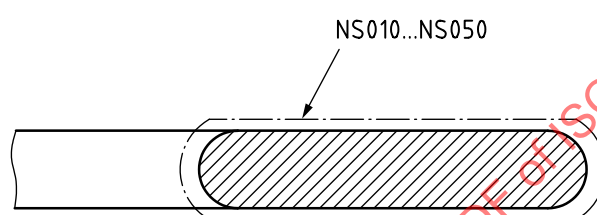
Figure 5 — Nitrided rail
