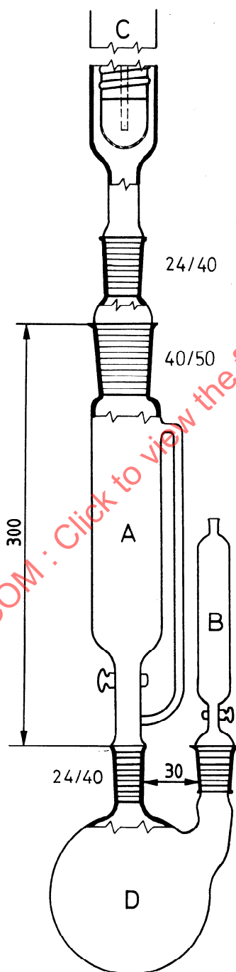
Figure 1 — Decomposition apparatus
