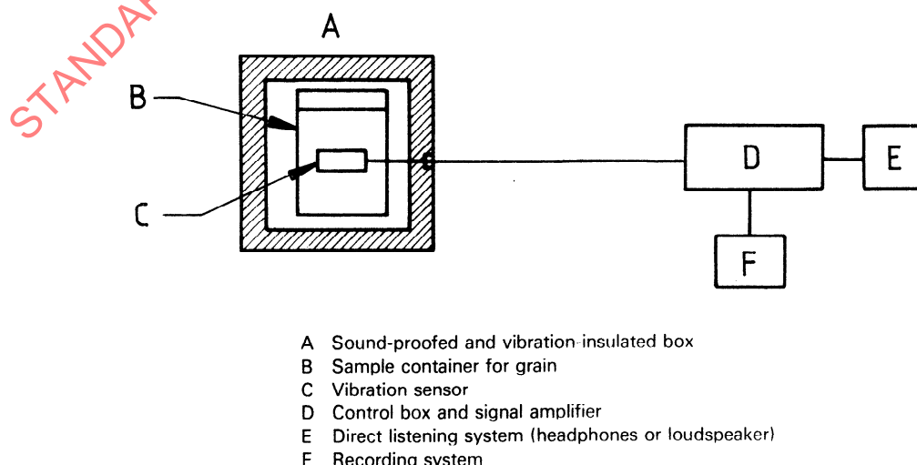
Figure 6 — Acoustic detection equipment
