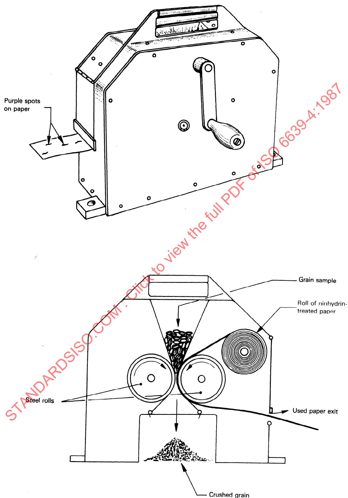
Figure 3 — Apparatus for ninhydrin detection of hidden insect infestation
