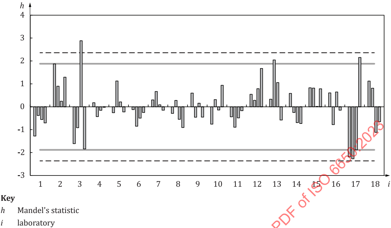
Figure B.3 — Mandel's interlaboratory consistency statistic, h , grouped by laboratories
