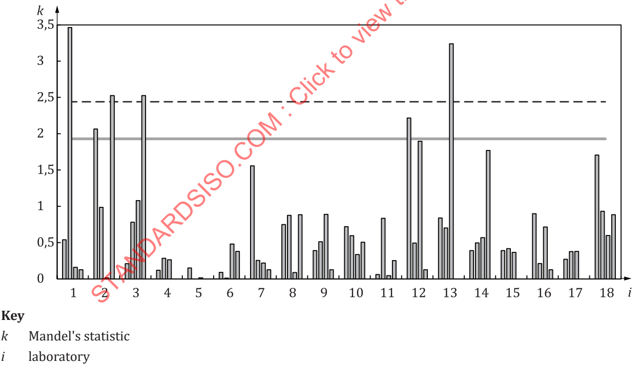
Figure B.4 — Mandel's intralaboratory consistency statistic, k , grouped by laboratories
