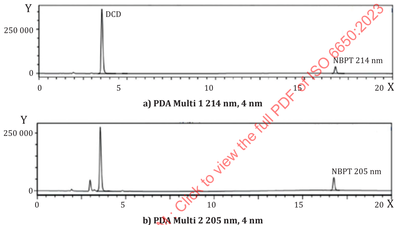
Figure A.1 — Typical HPLC chromatogram of DCD and NBPT of a urea-based fertilizer
