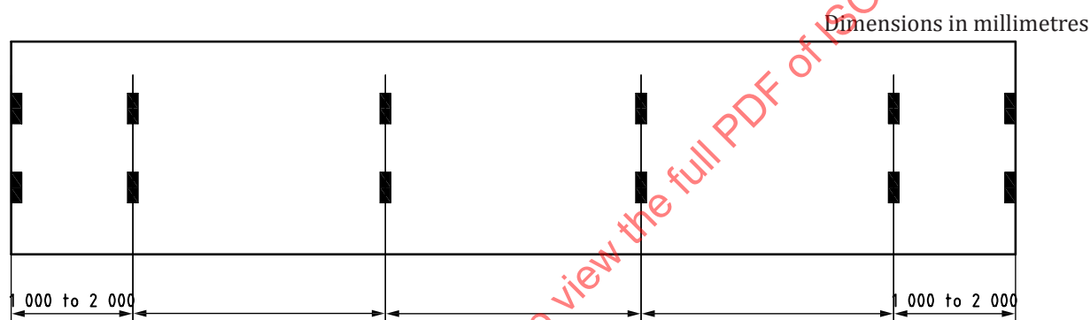
Figure B.6 — 1AA, 1A or 1AX containers without gooseneck tunnel — Minimum requirements
