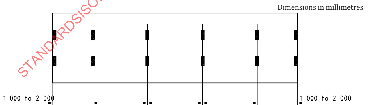
Figure B.4 — 1BBB, 1BB, 1B or 1BX containers — Minimum requirements
