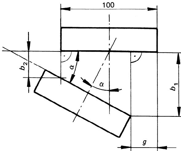
Figure 8 — Measurement of eccentricity
