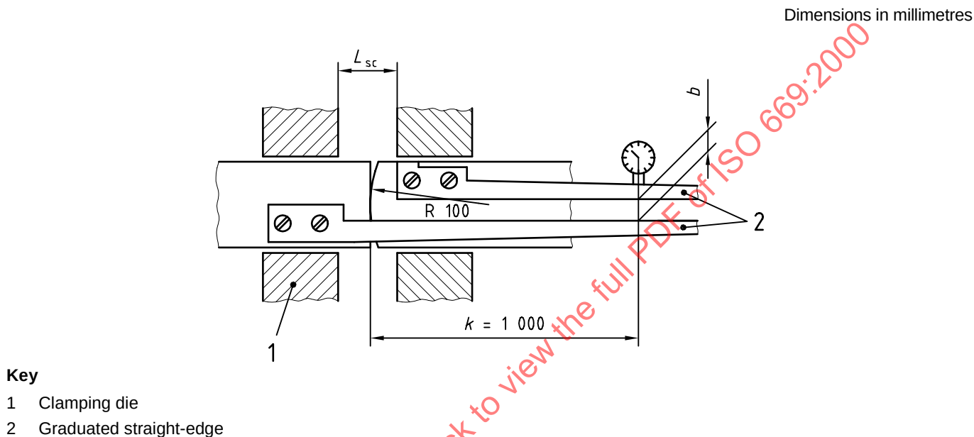
Figure 19 — Measurement arrangement for butt welding equipment
