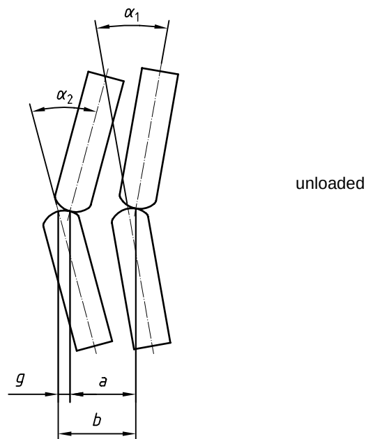
Figure 11 — Contact fault of spot and seam welding equipment
