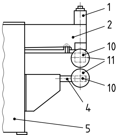
longitudinal seam welding equipment
