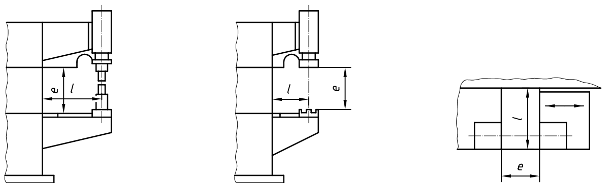
a) spot welding equipment
