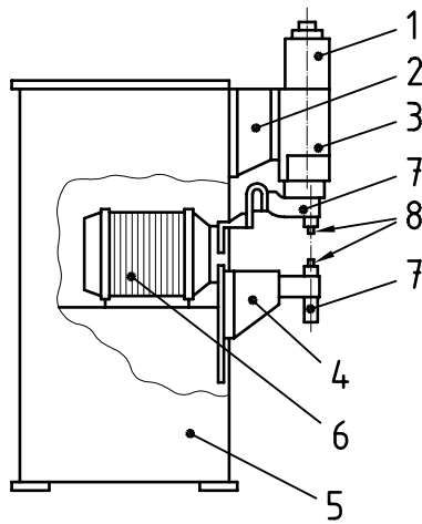
a) spot welding equipment
