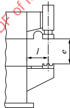
b) Projection welding equipment
