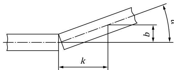
Figure 11 — Contact fault of upset welding equipment
