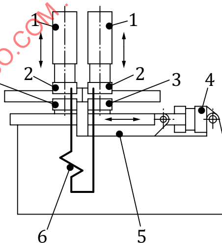
Figure 1 — Elements of spot, projection, and seam welding equipment
