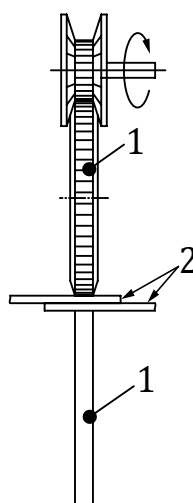
b) Knurl drive
