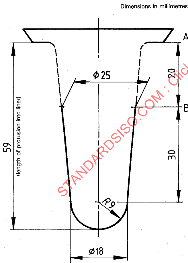
Figure 1 – Teatcup plug
