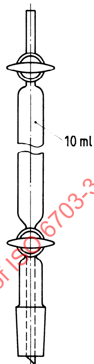
Figure 4 — 10 ml sampling funnel
