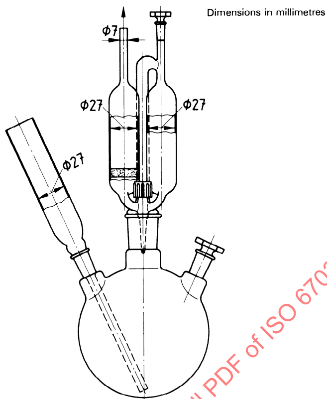
Figure 1 — Three-necked distillation flask
