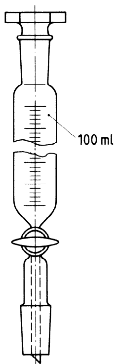
Figure 3 — Separating funnel
