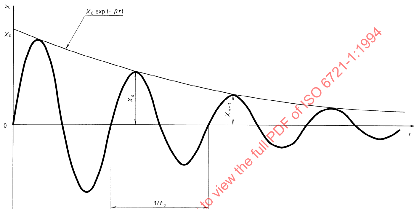
Figure 3 — Damped-vibration curve for a viscoelastic system undergoing freely decaying vibrations
