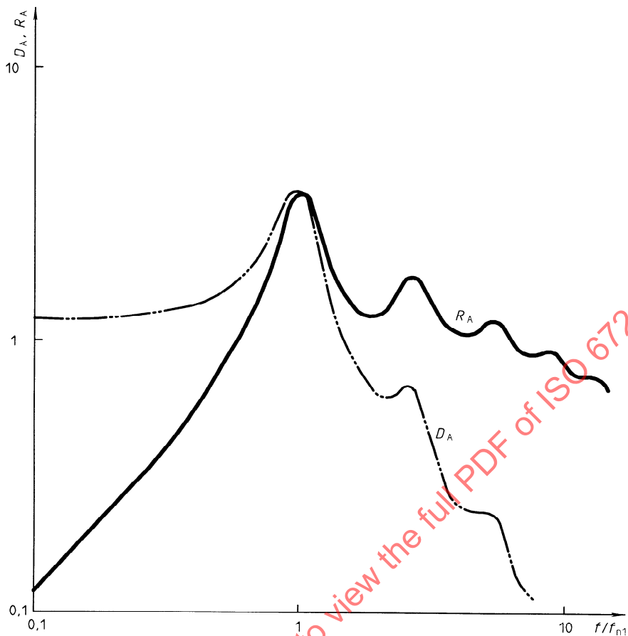
Figure A.4 — Multiple resonance curves as in figures A.2 and A.3 with \tan \delta = 0,6
