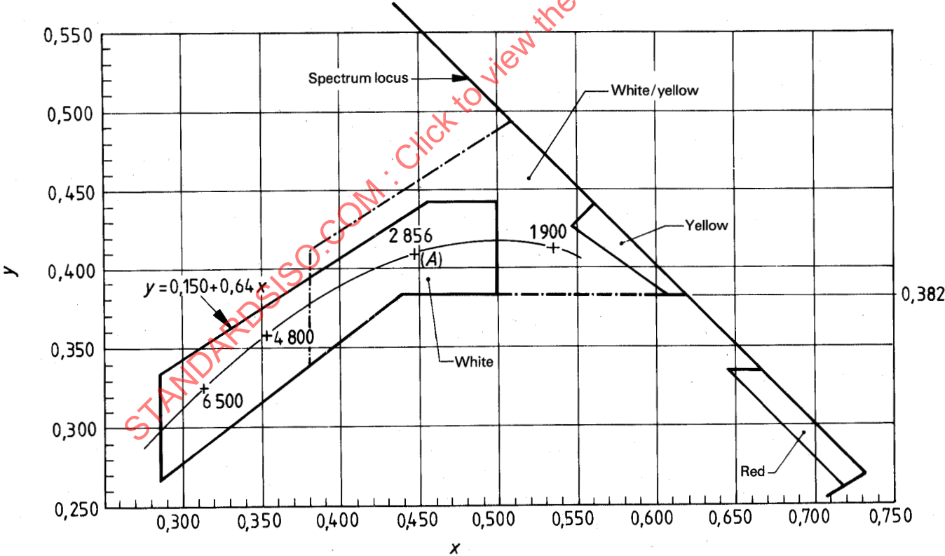
Figure 2 — Boundaries of colour areas for reflective devices
