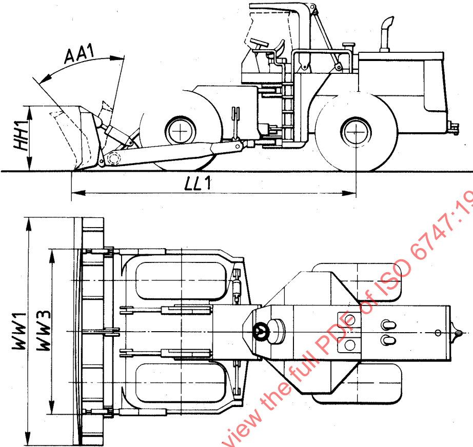
Figure 16 — Dimensions of dozer equipment (wheel tractor)
