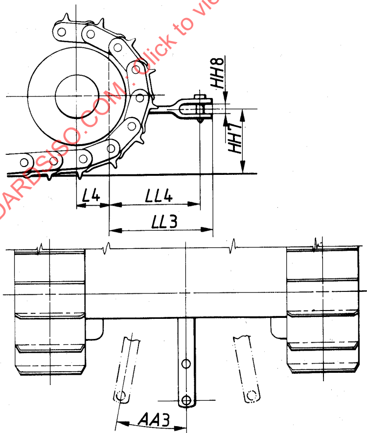
Figure 19 — Dimensions of swinging drawbar
