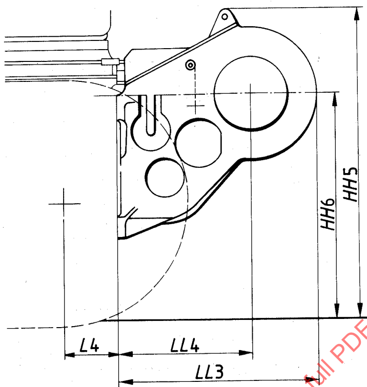
Figure 18 — Dimensions of winch equipment
