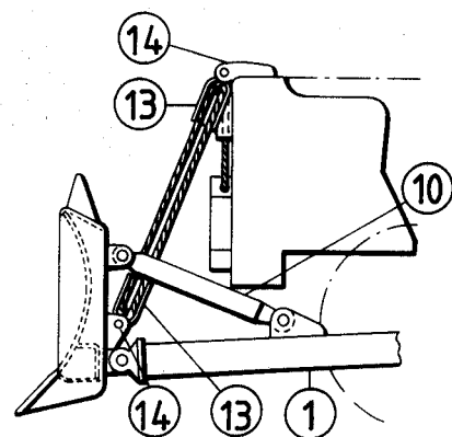
Angling blade
