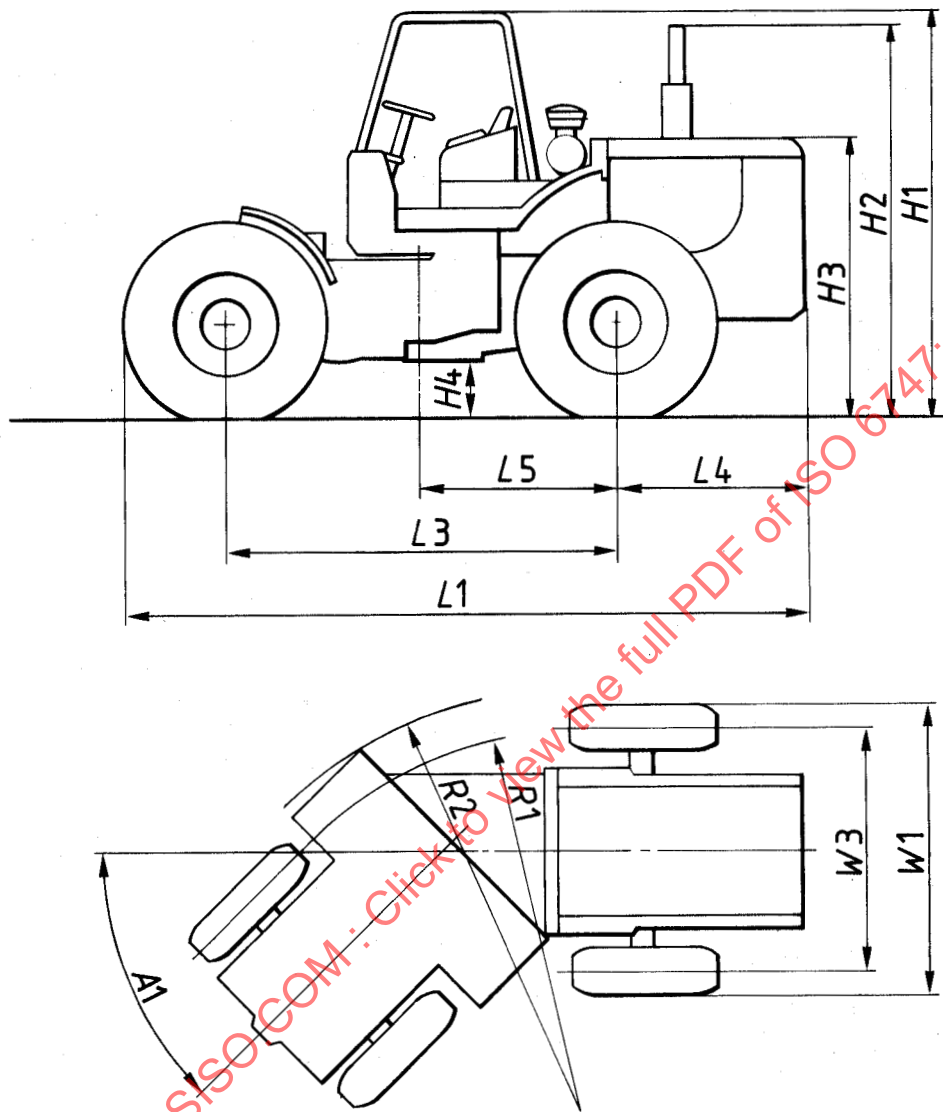
Figure 7 — Dimensions of base machine (wheel tractor)
