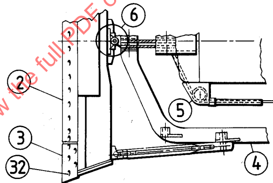
Angling blade
