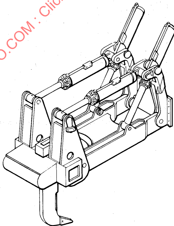
Figure 22 — Ripper — Variable type
