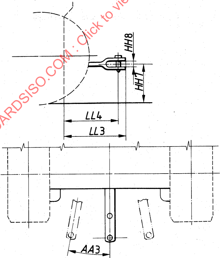
Figure 27 — Dimensions of swinging drawbar
