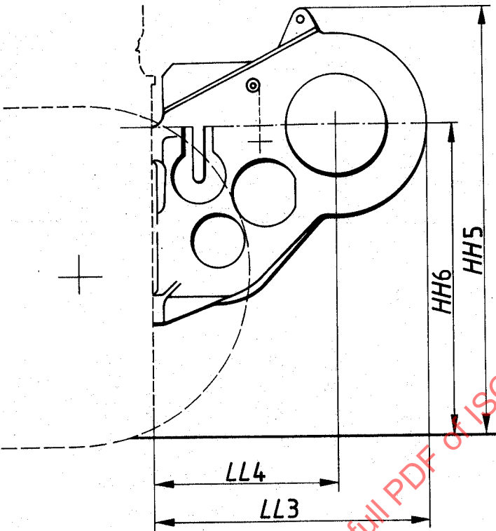
Figure 26 — Dimensions of winch equipment
