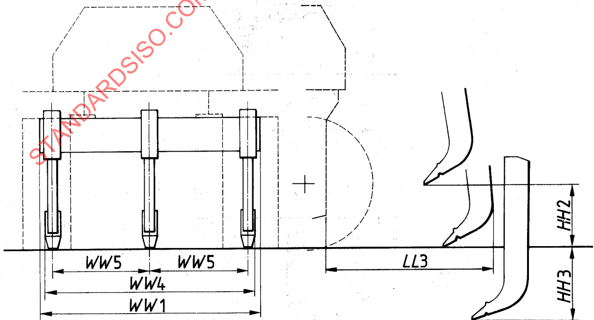
Figure 25 — Dimensions of ripper
