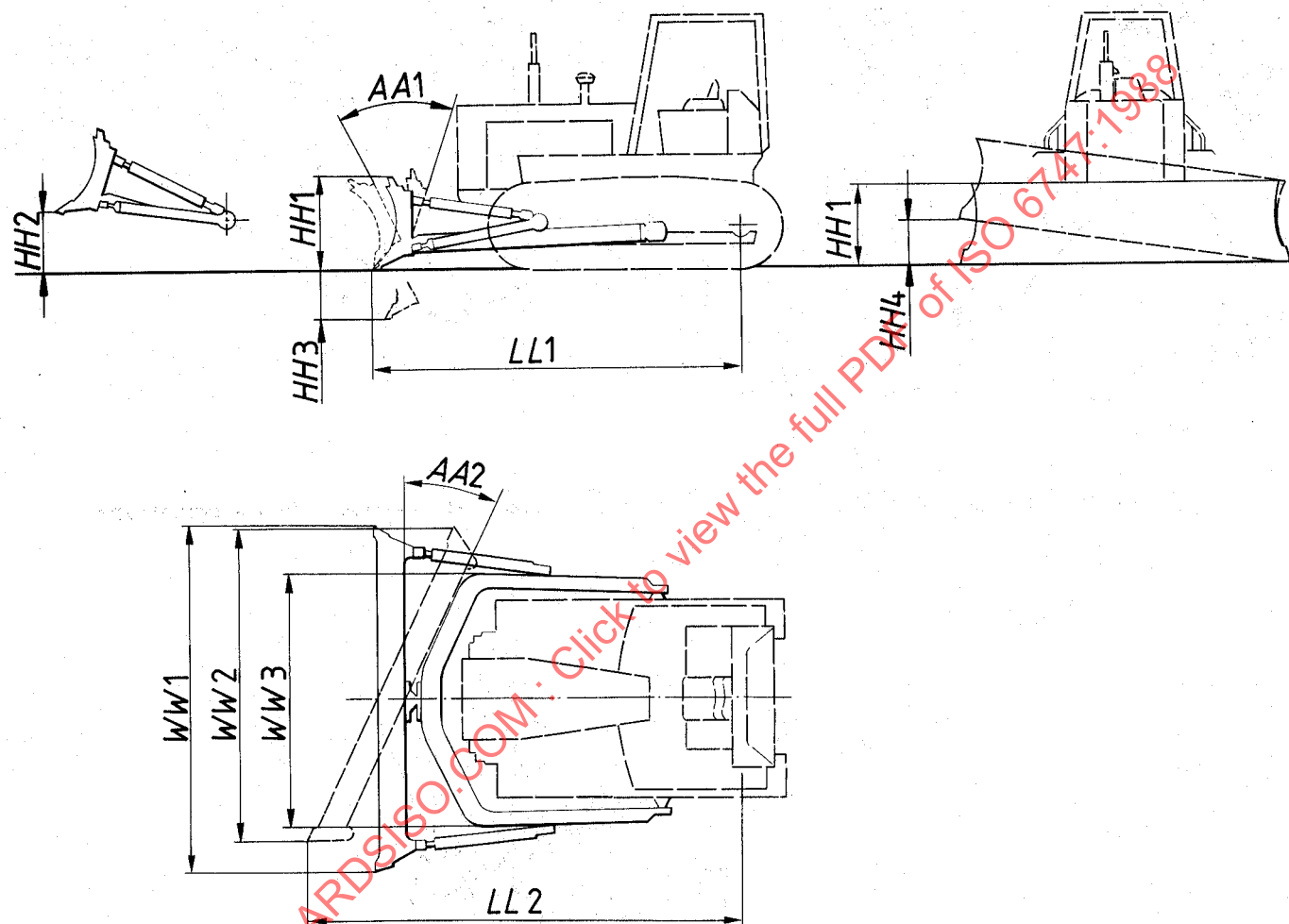
Figure 23 — Dimensions of dozer (crawler tractor)
