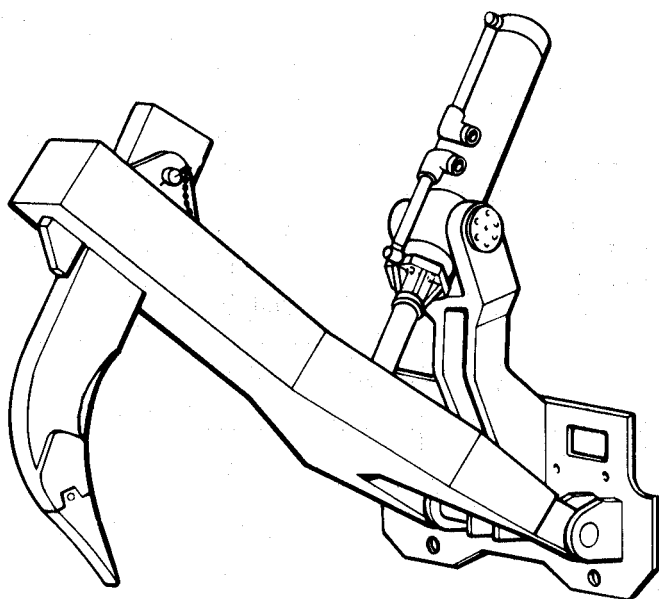
Figure 20 — Ripper — Radial type
