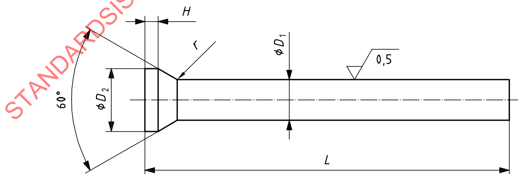
Figure 1 — Round punches with 60° conical head and straight shank
