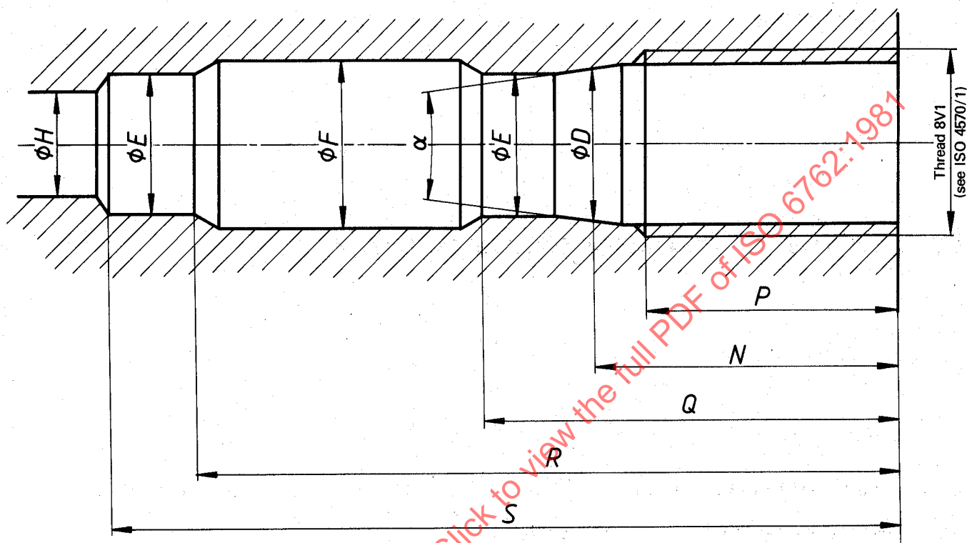
Figure 1 — Core chamber
