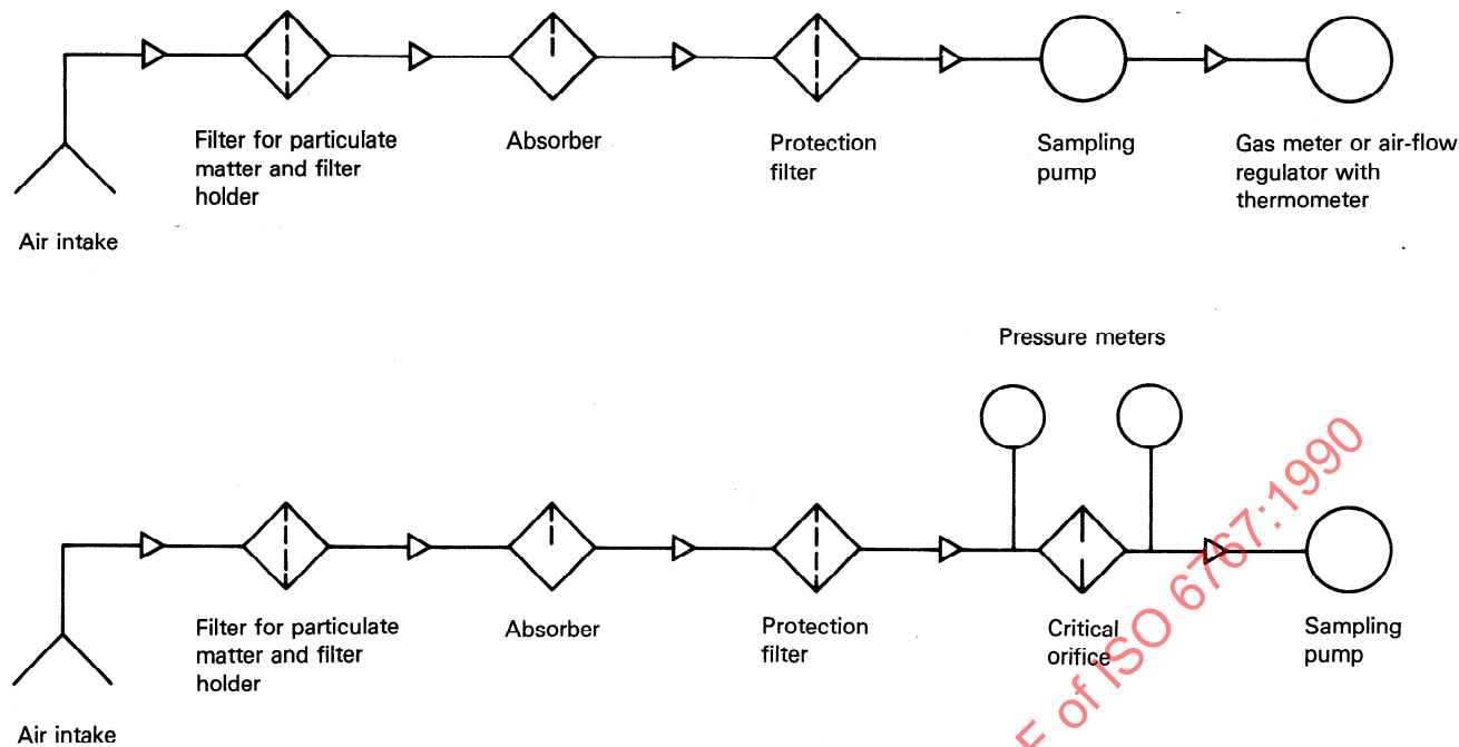
Figure 2 — Examples of sampling trains for the determination of the mass concentration of sulfur dioxide in ambient air
