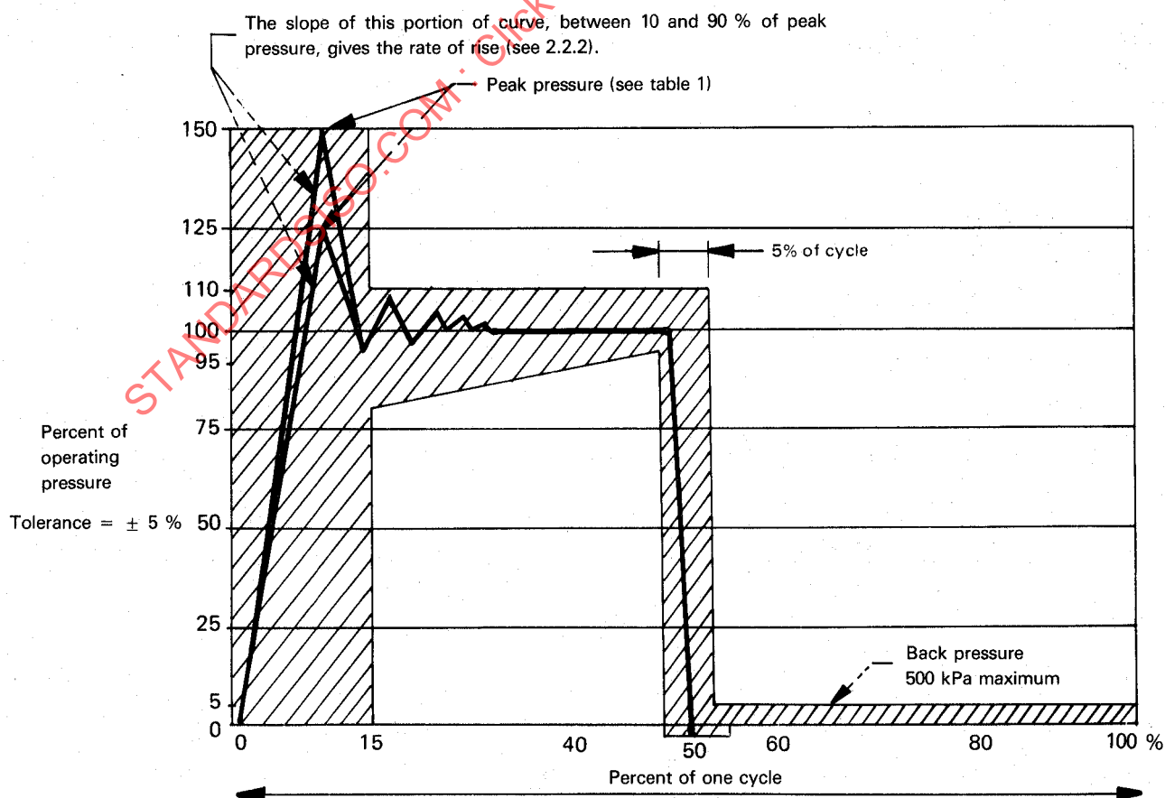
Figure 1 — Impulse trace
