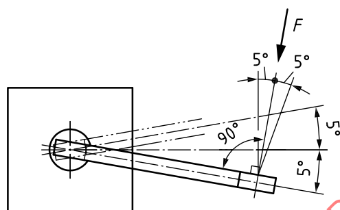
a) Wrench in a horizontal position
